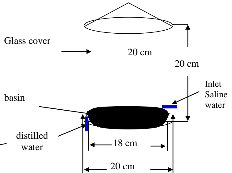
Figure 2: A schematic diagram of the Hemispherical Solar Still (HSS)
